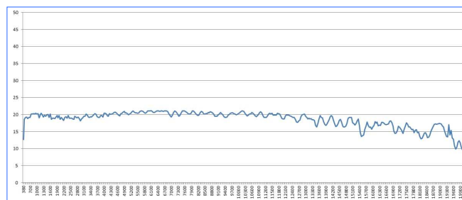
Gain diagram HyperLOG 30200X
