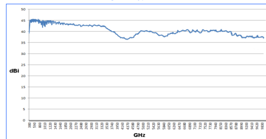
Gain diagram HyperLOG 30100X
