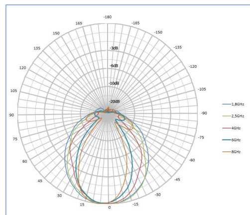
Vertical Pattern HyperLOG 30 X Series
